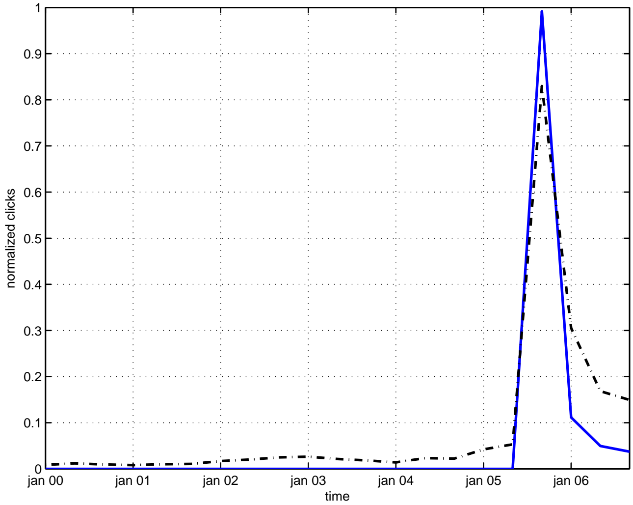
dipole instanton
