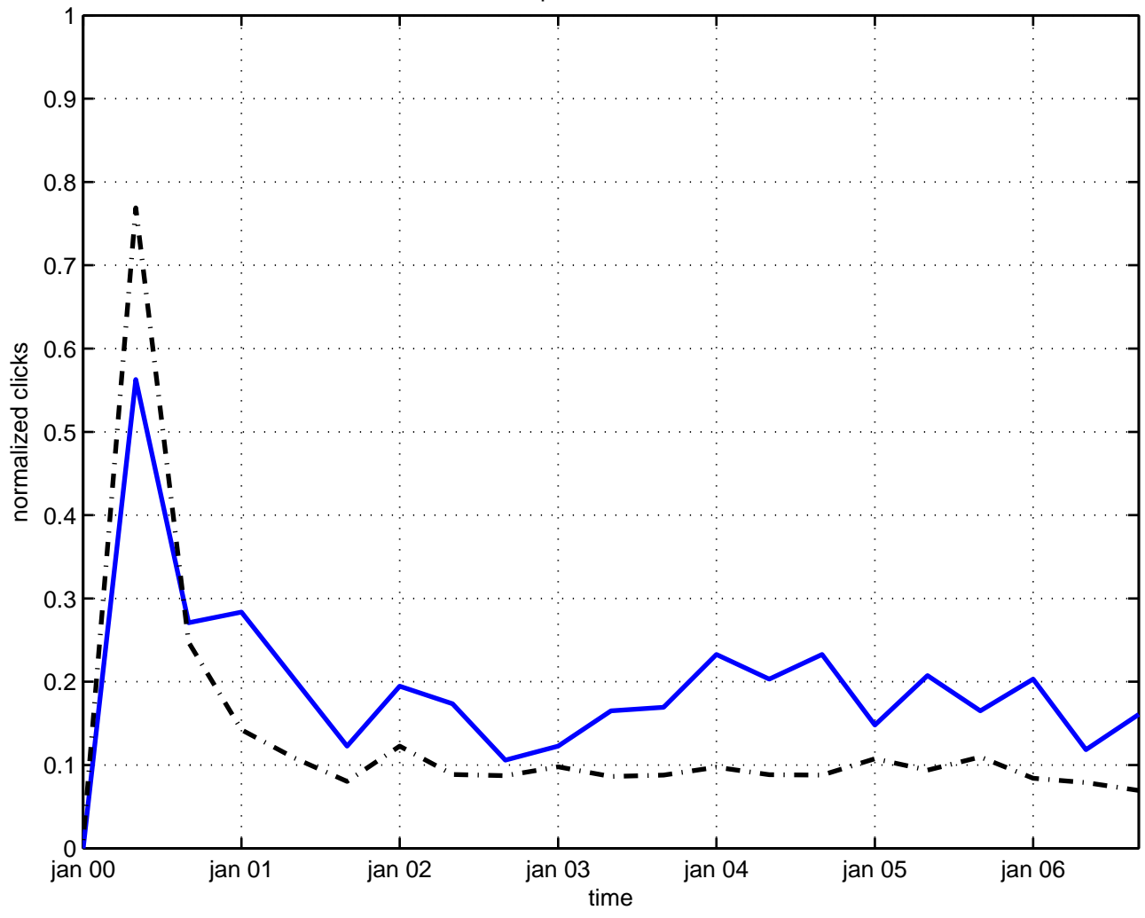
dipole fluctuation
