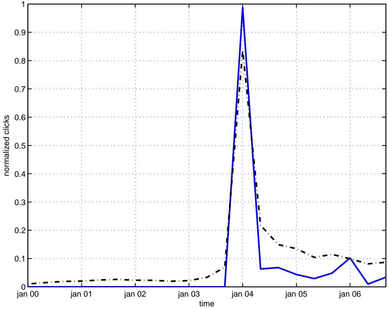
dimension fractal
