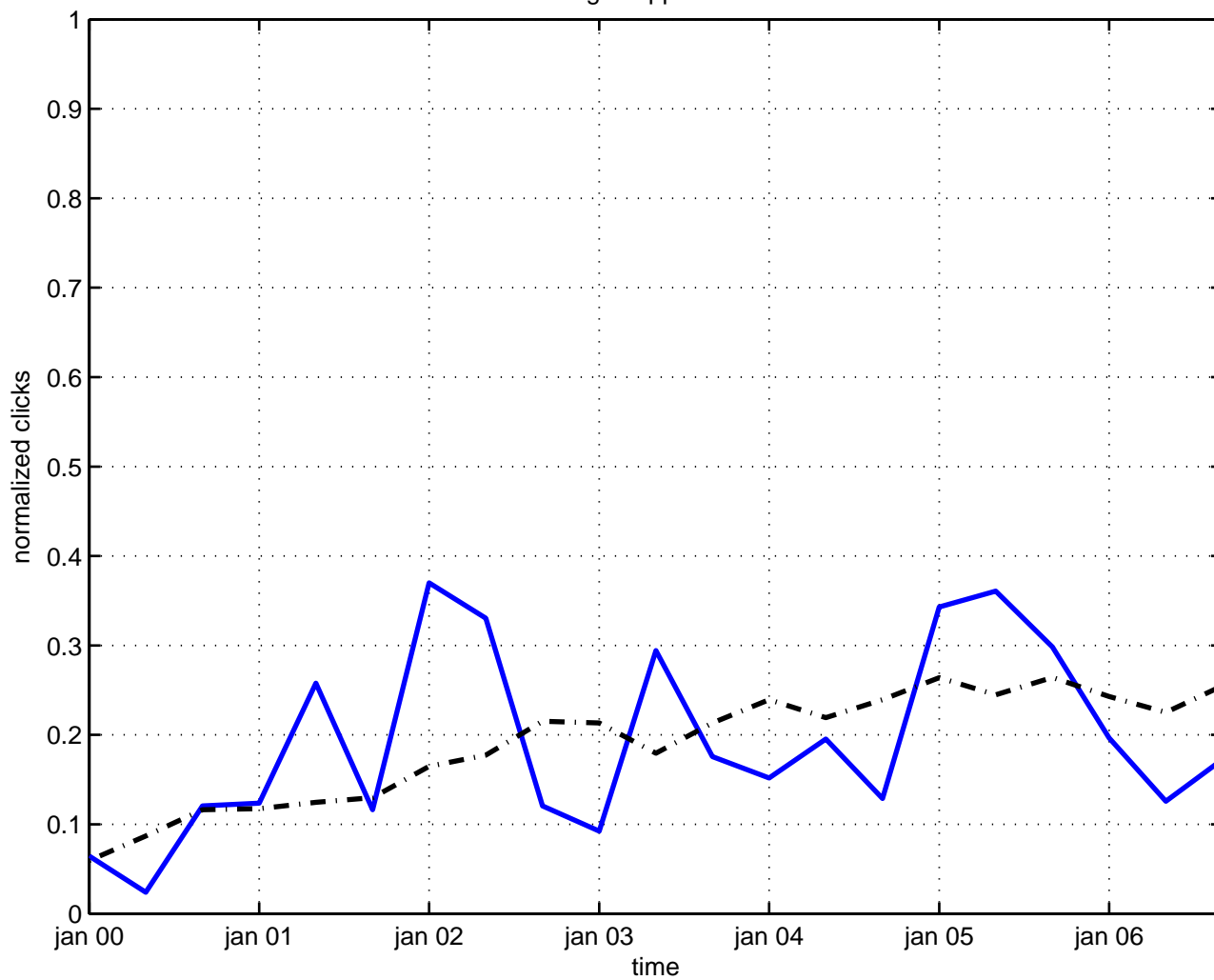
dilute gas approximation
