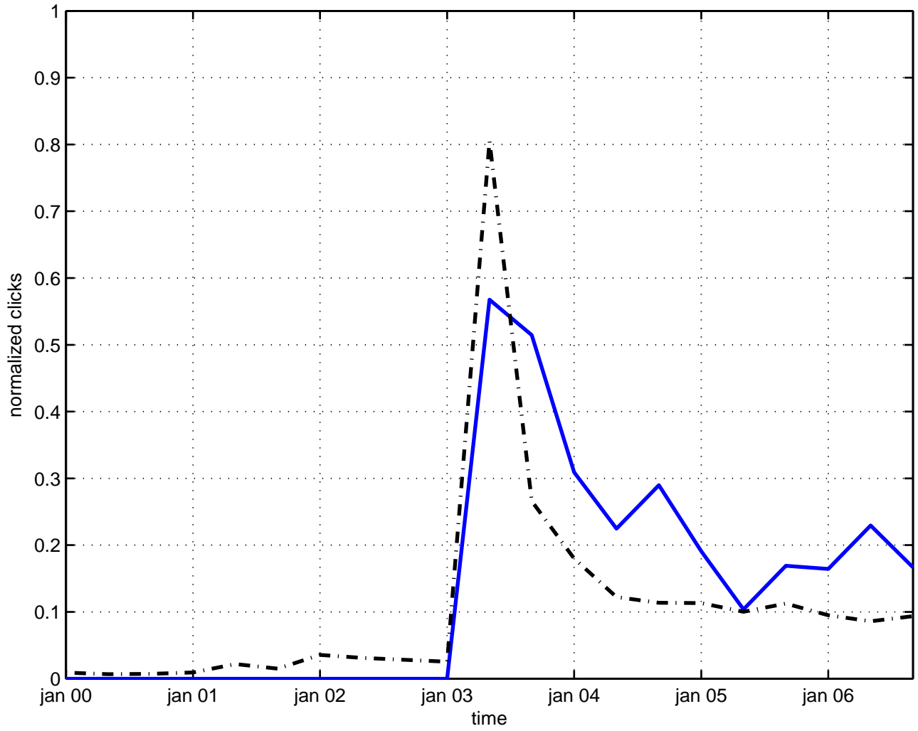
dilation symmetry
