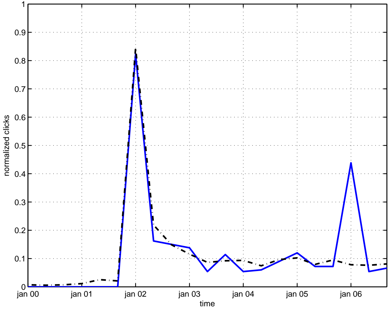
differential renormalization
