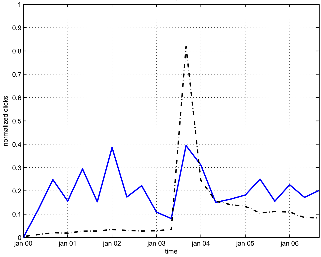
diffeomorphism
