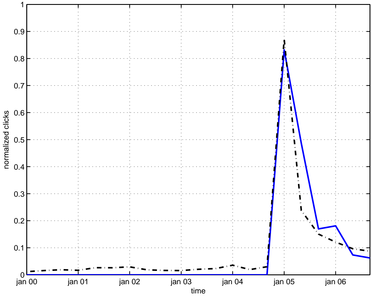
diffeomorphism anomaly
