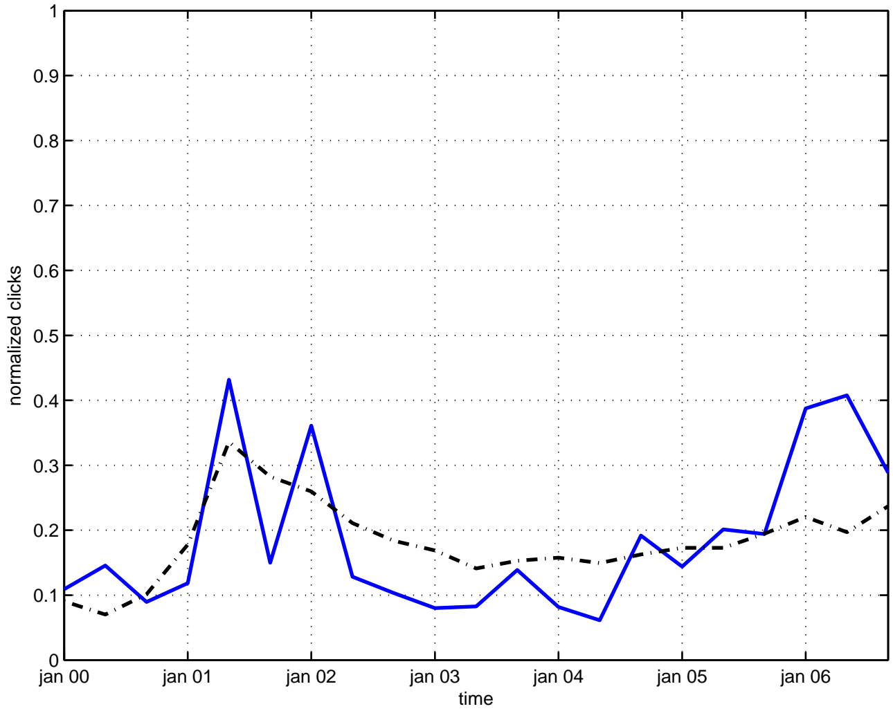
determinant
