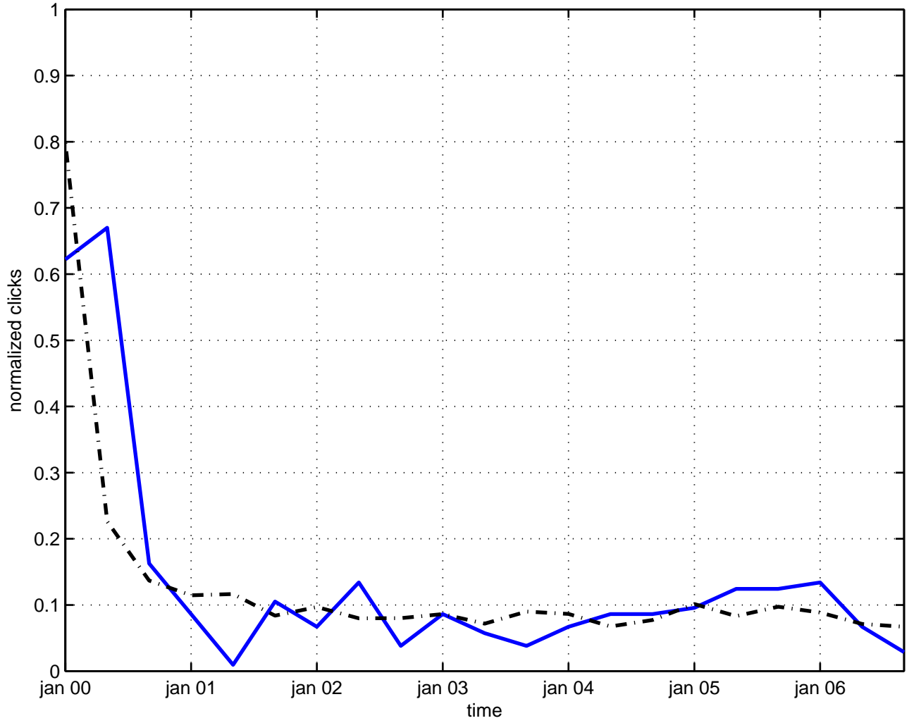
determinant quaternion
