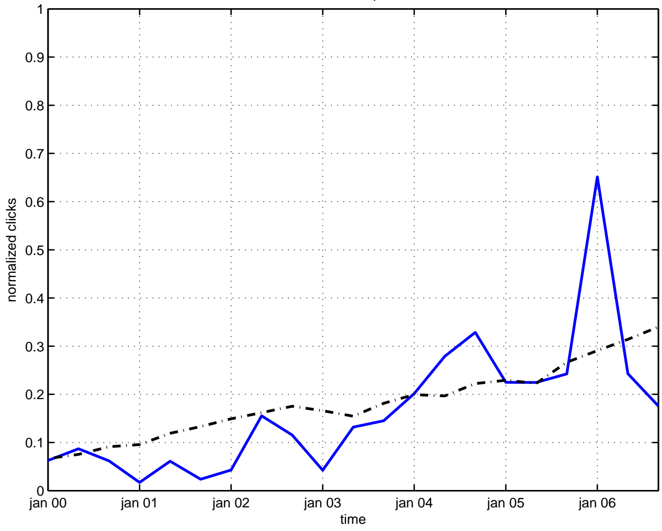
determinant operator
