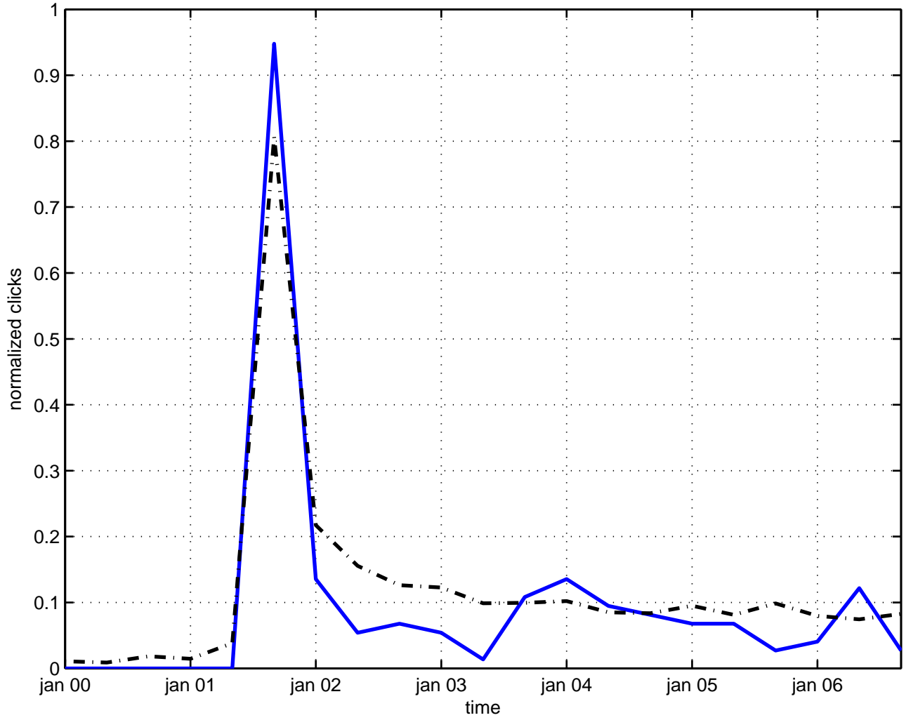
derivative dispersion relation
