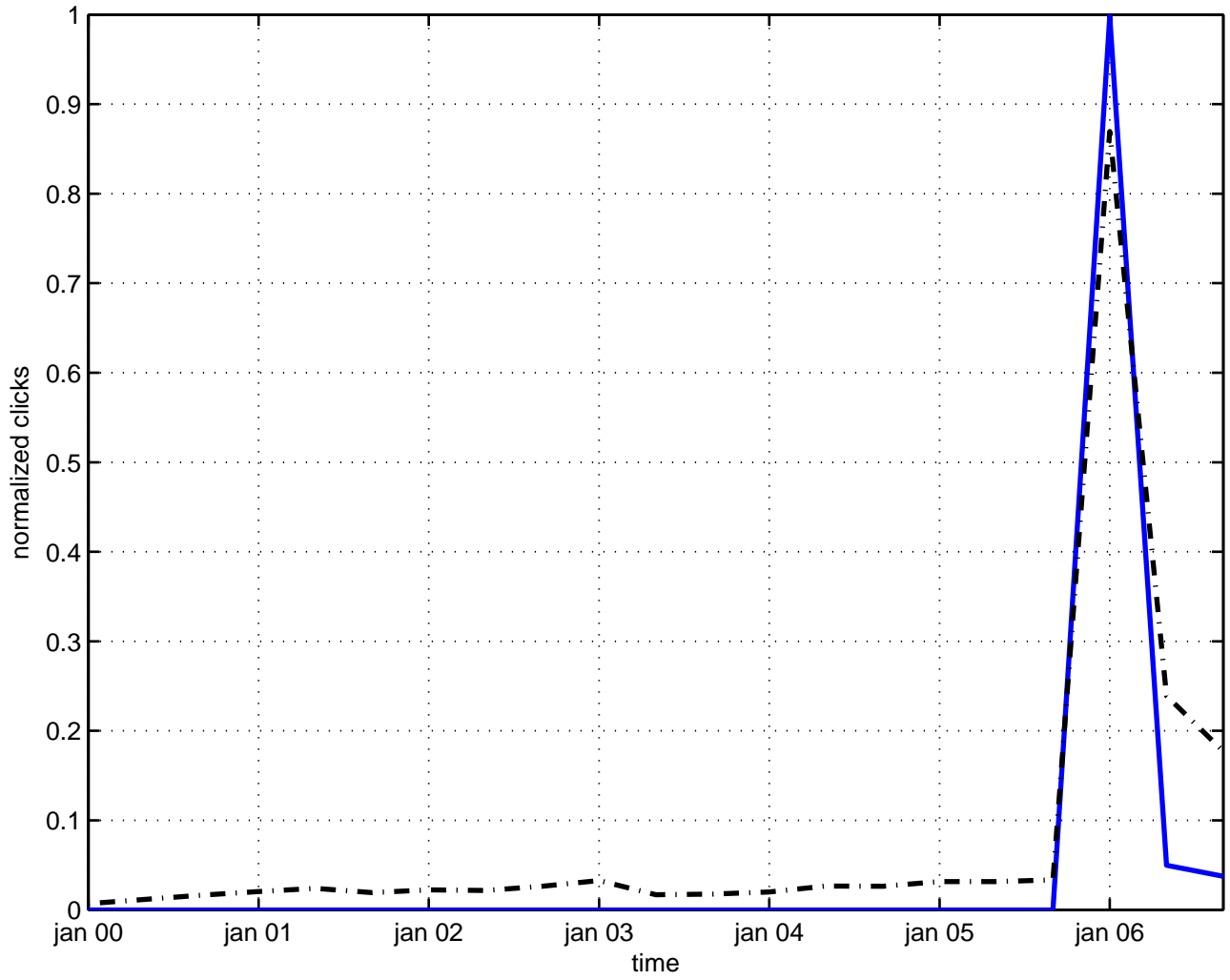
derivative coupling
