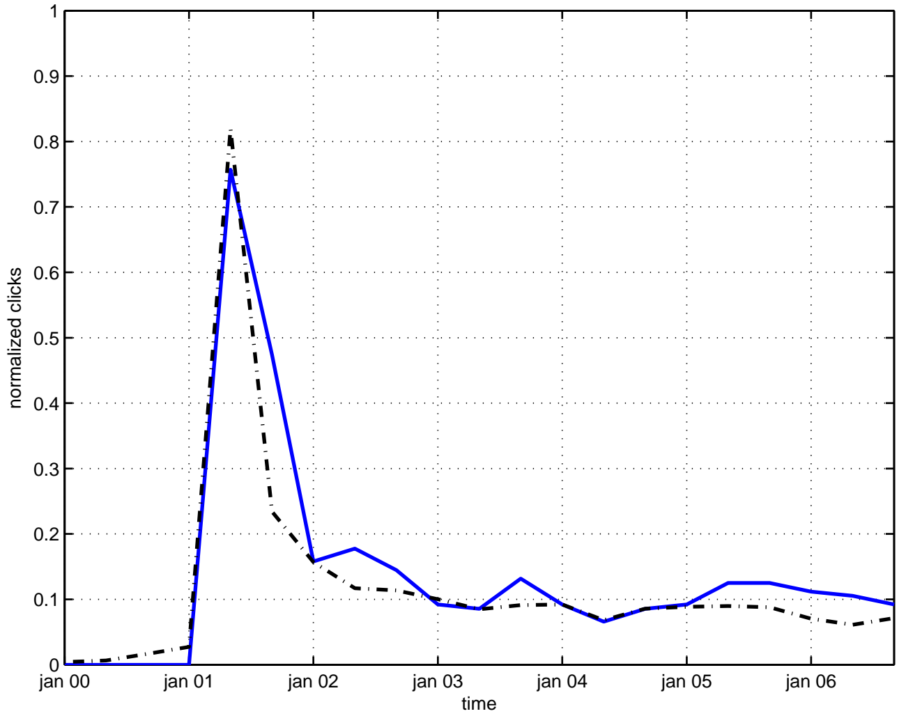
dependence scaling
