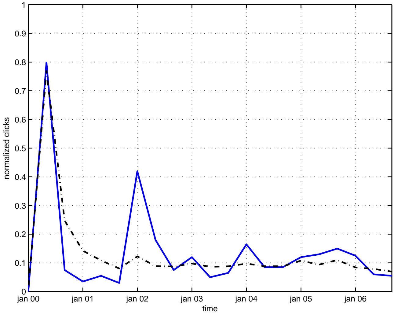
dependence renormalization
