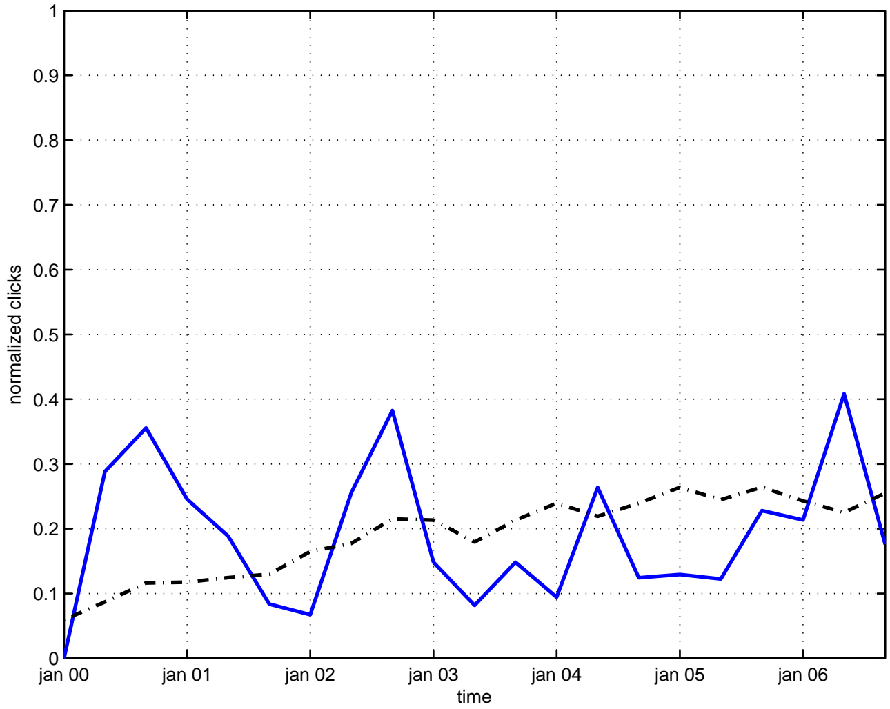
dependence regularization
