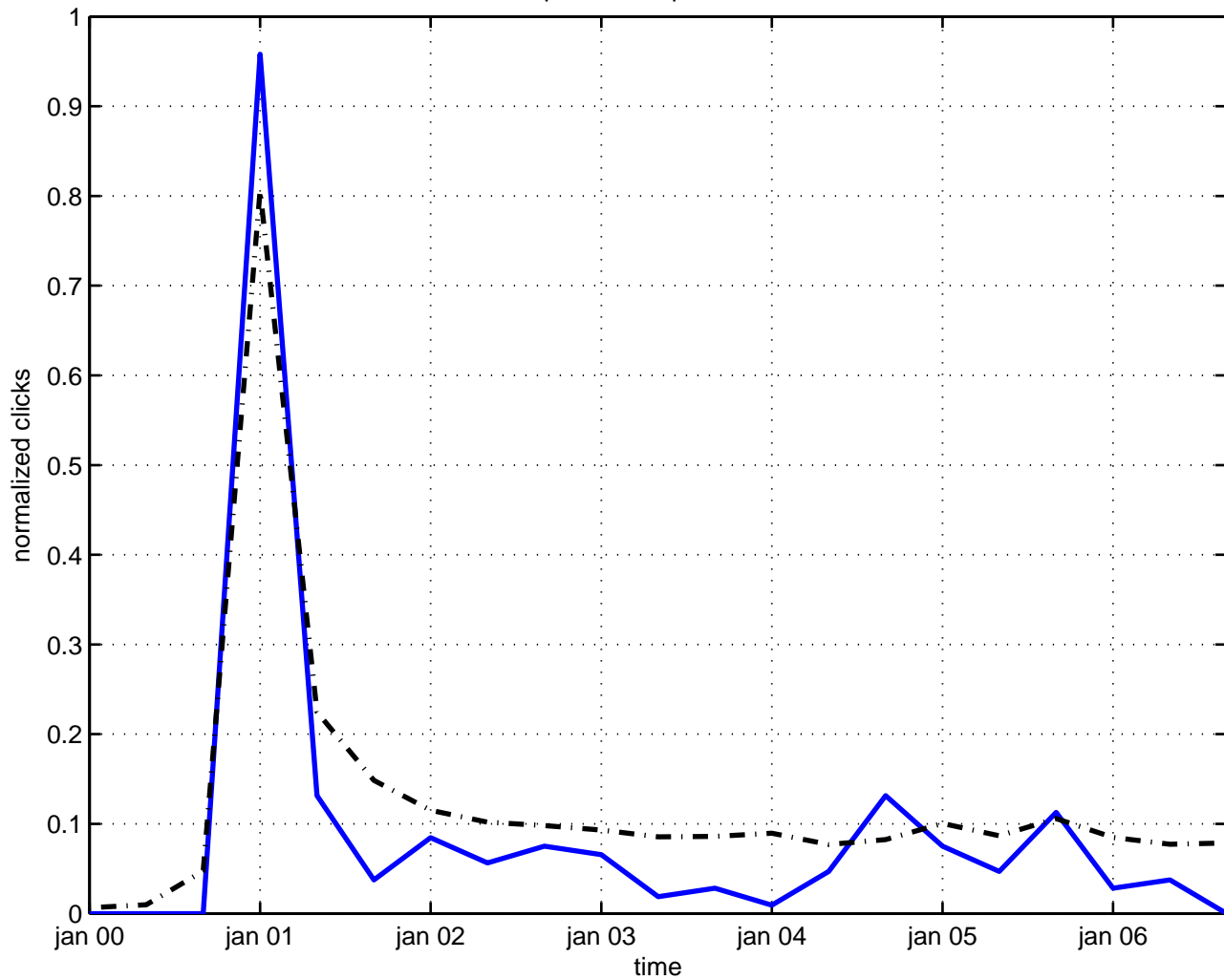
dependence quantization
