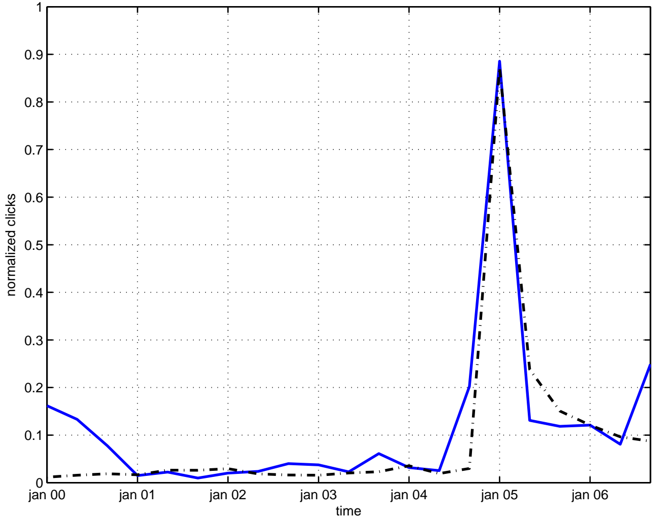
dependence dimension
