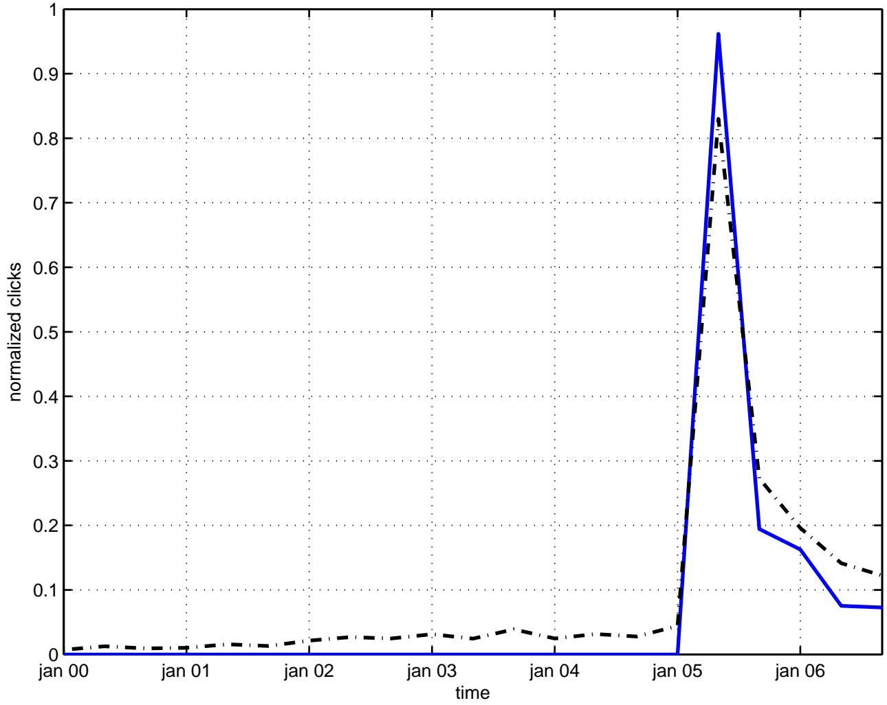
dependence cosmological constant
