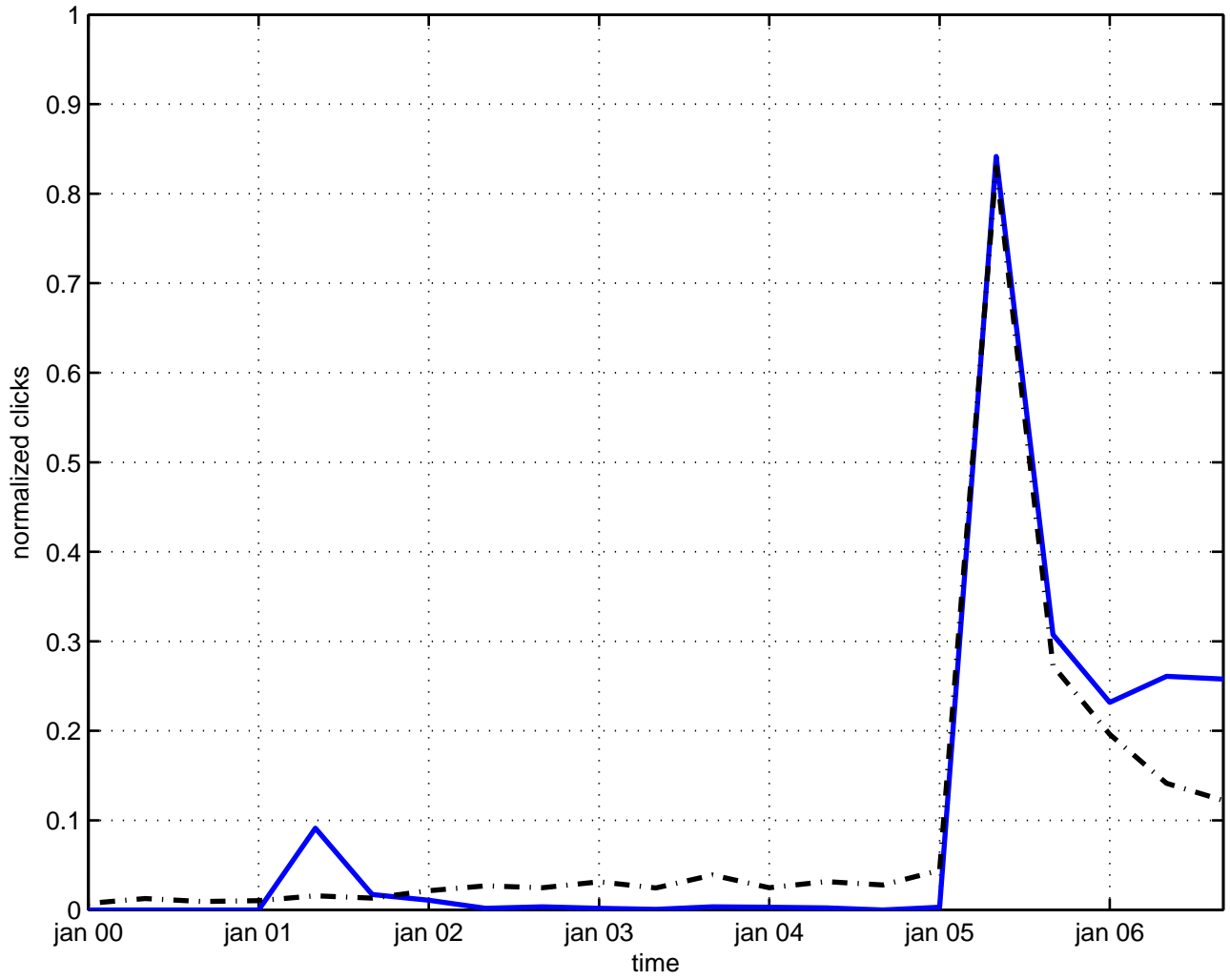
dependence background field
