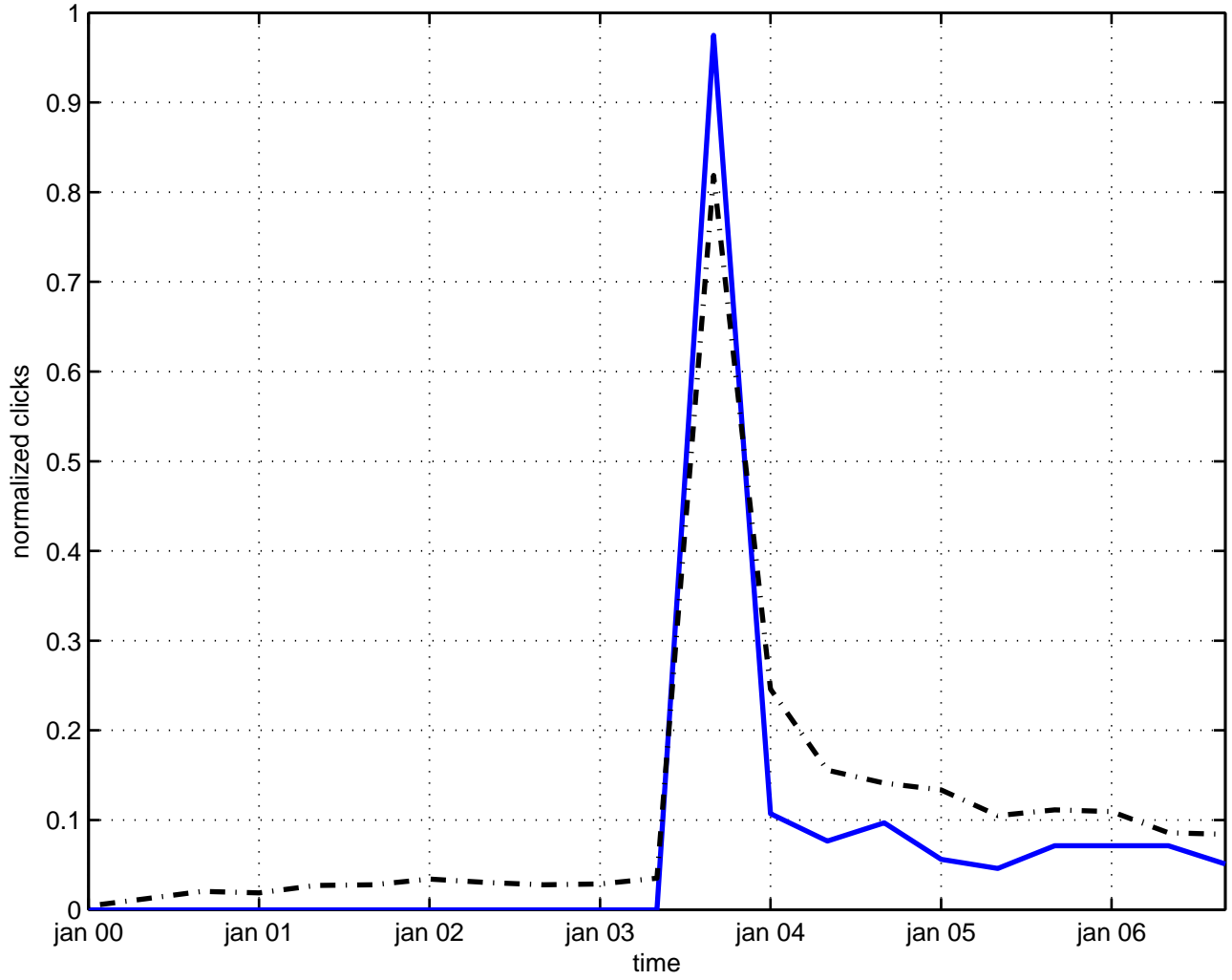
density momentum
