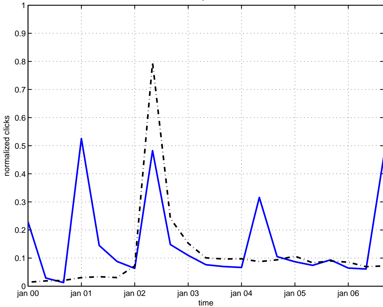
density matter
