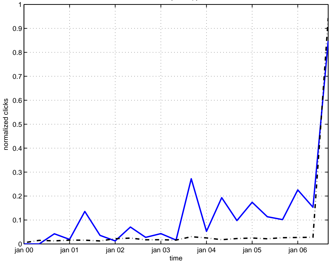
density entropy
