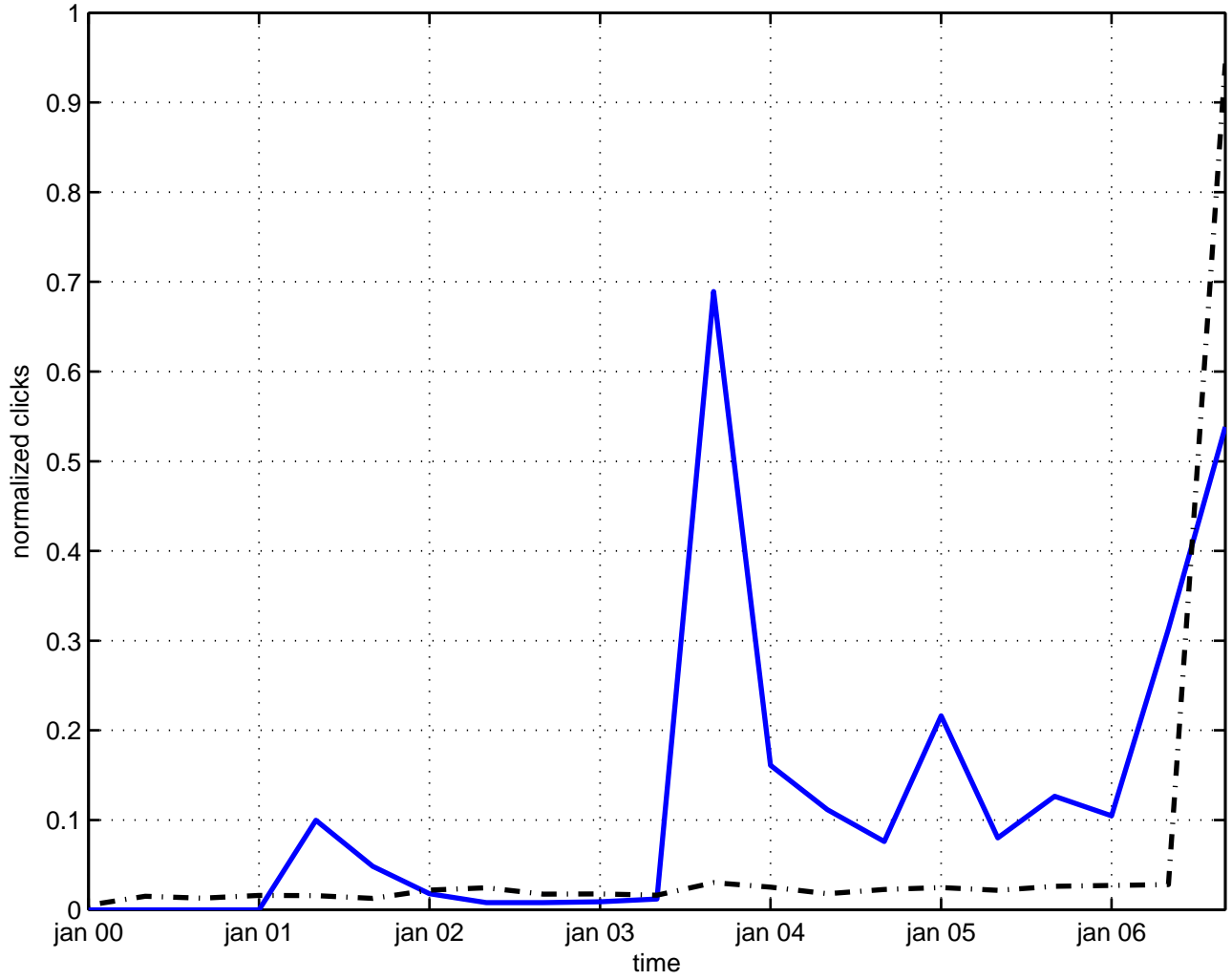
density dark energy
