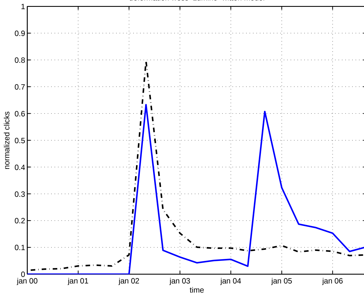
deformation wess-zumino-witten model
