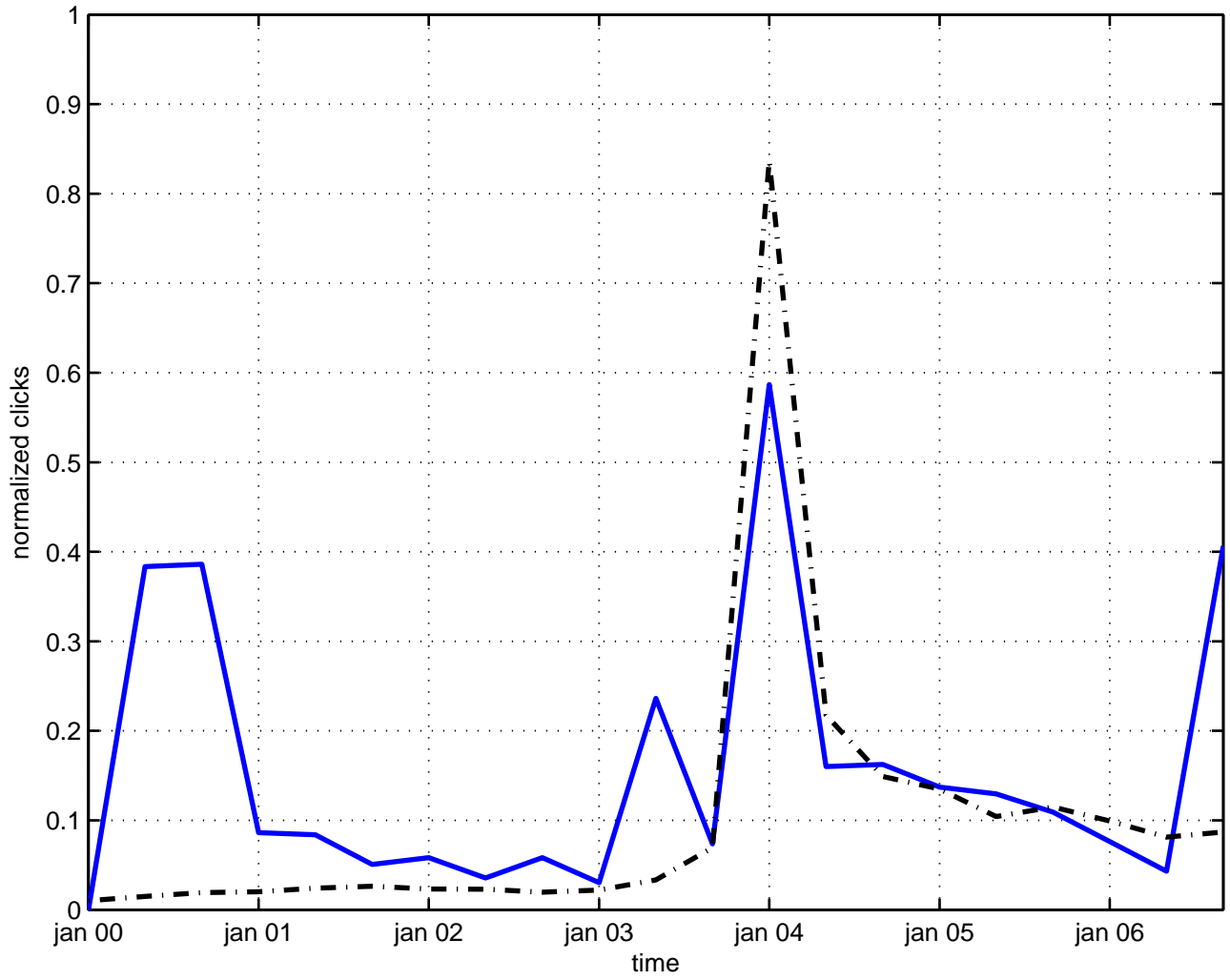
deformation transformation
