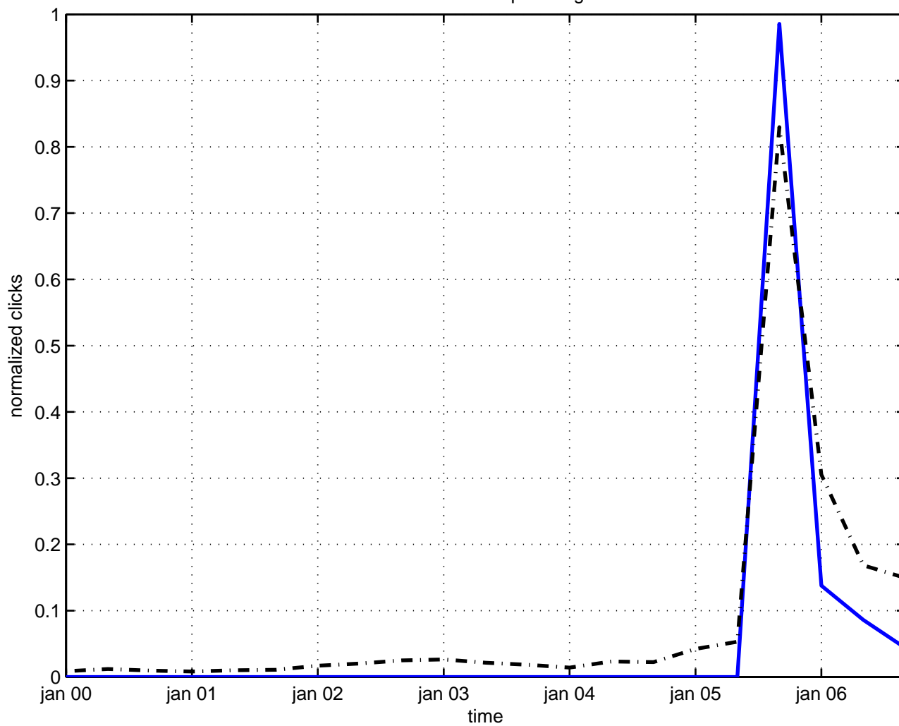
deformation superstring
