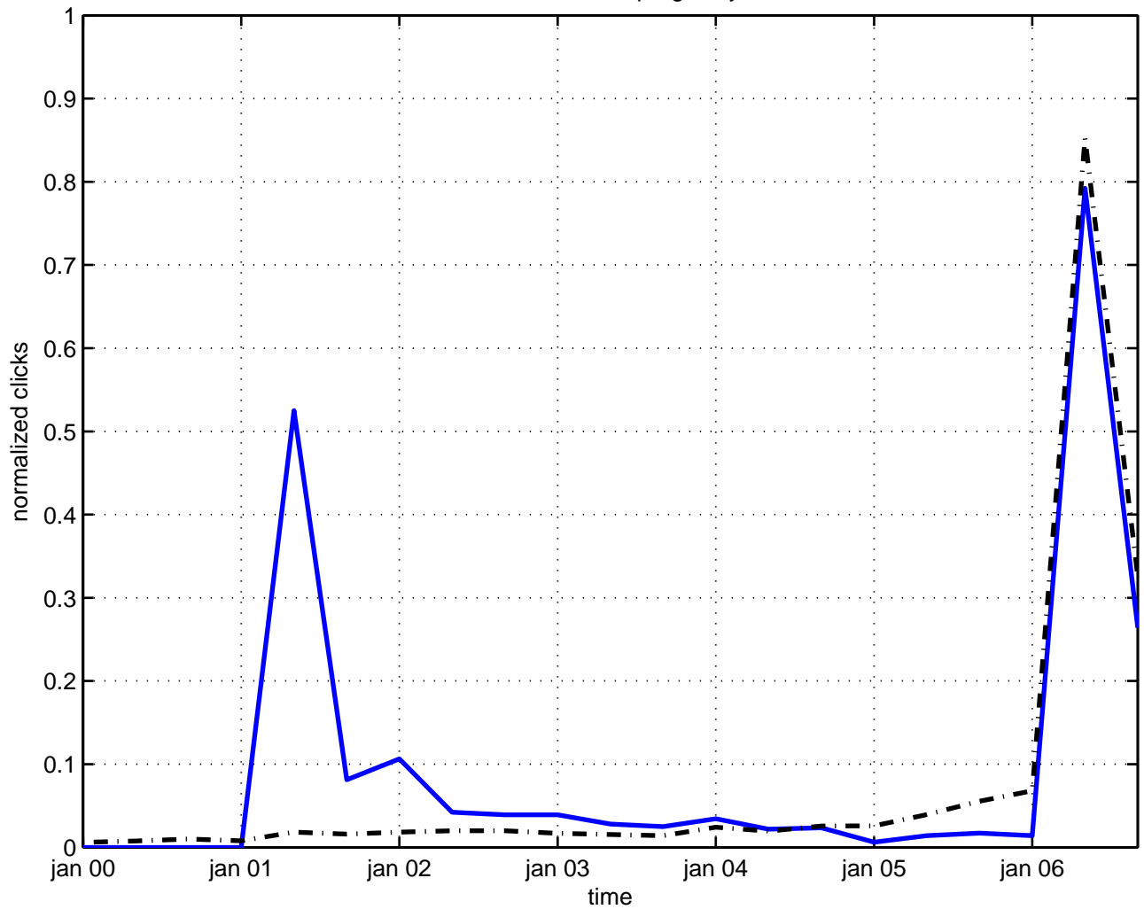
deformation supergravity
