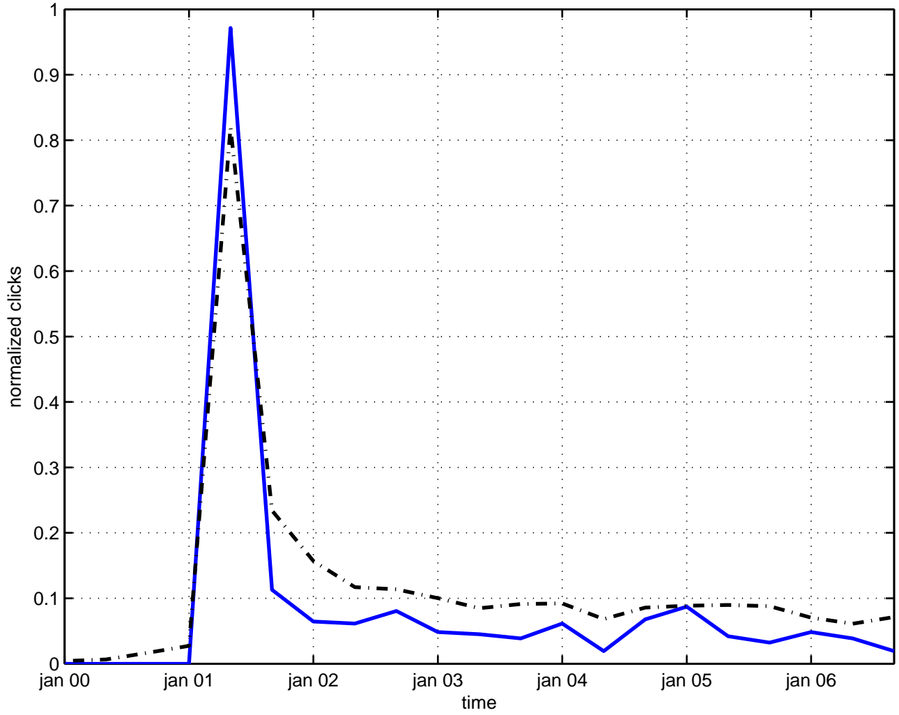
deformation quantum electrodynamics
