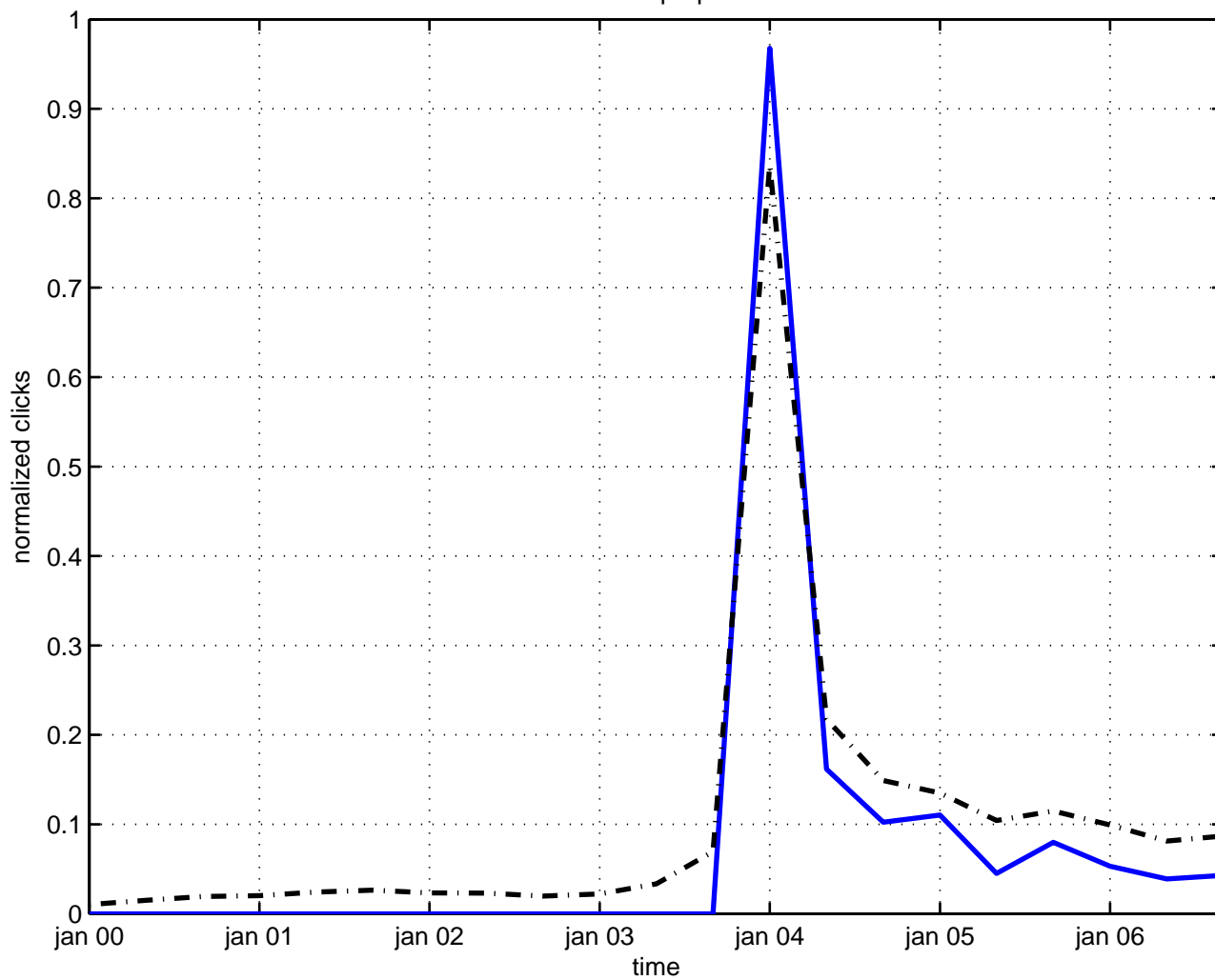
deformation prepotential
