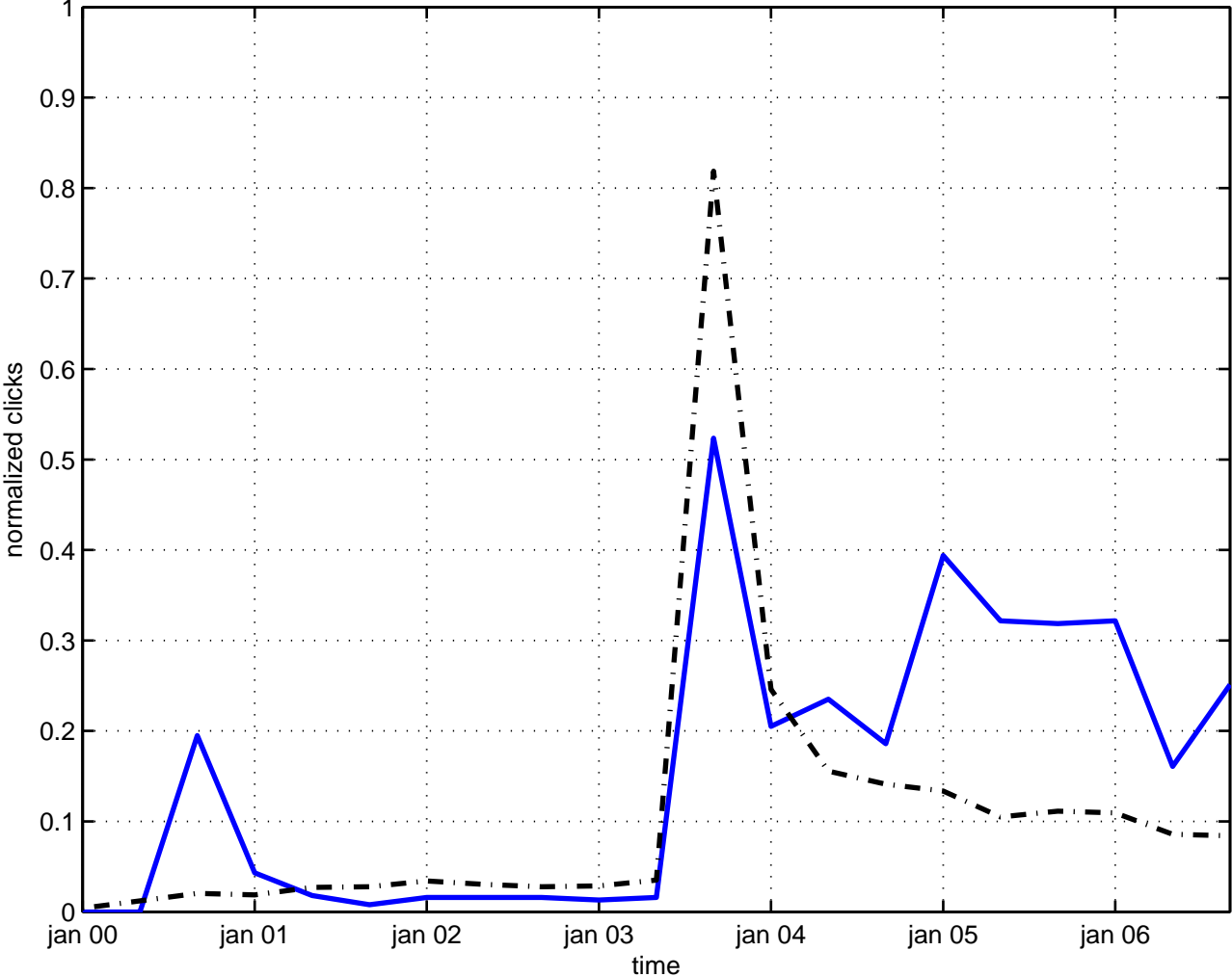
deformation group theory
