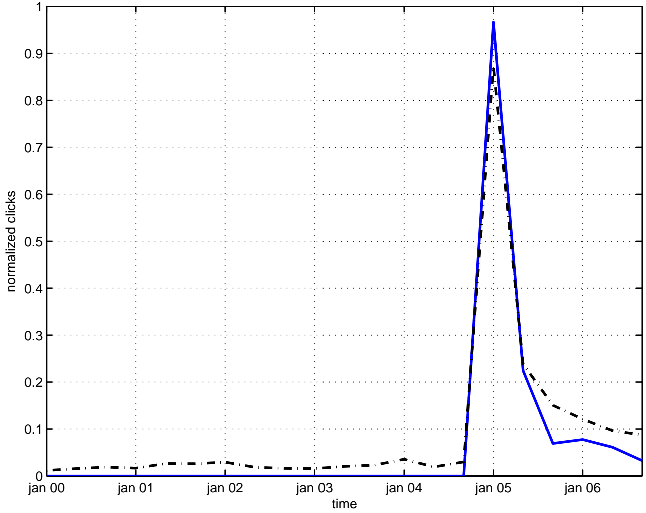
deformation dilaton
