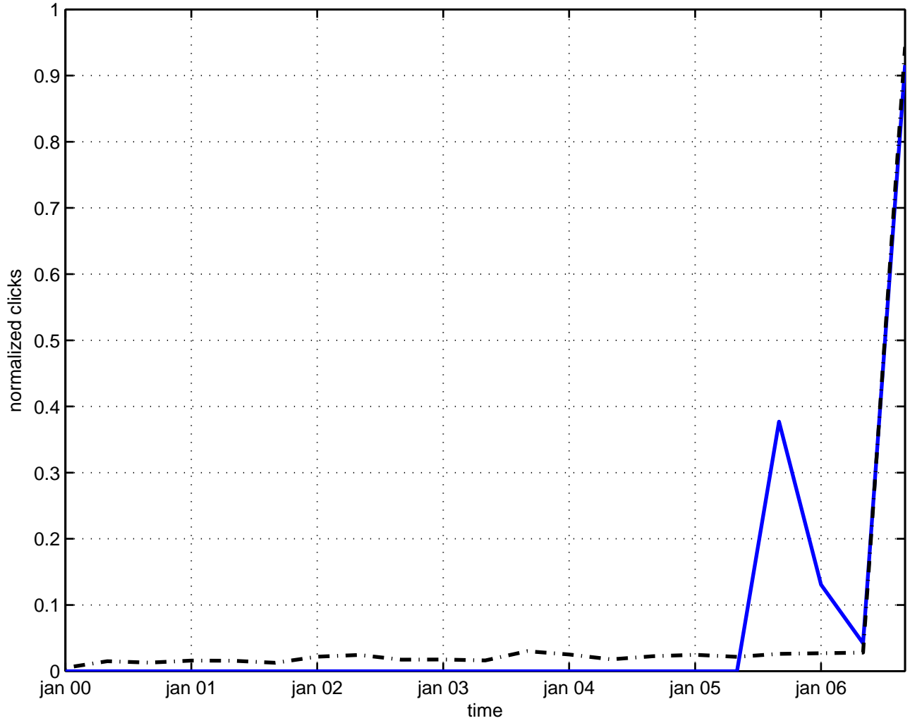
deformation black hole
