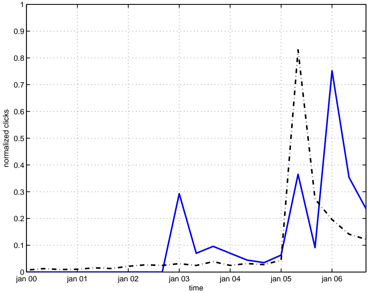
defect space-time
