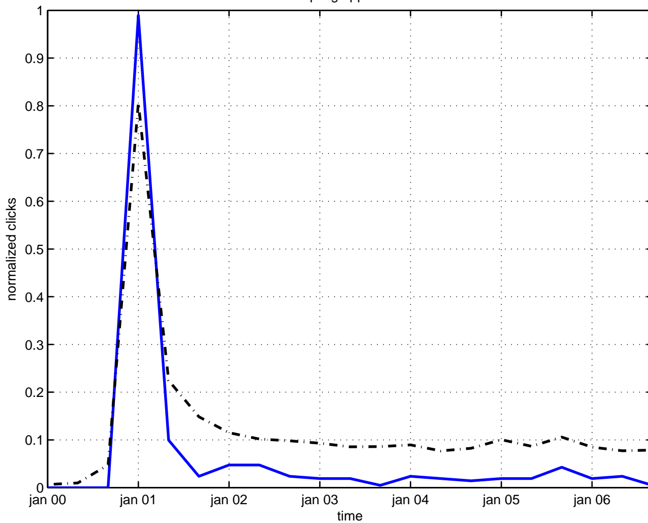
decoupling approximation
