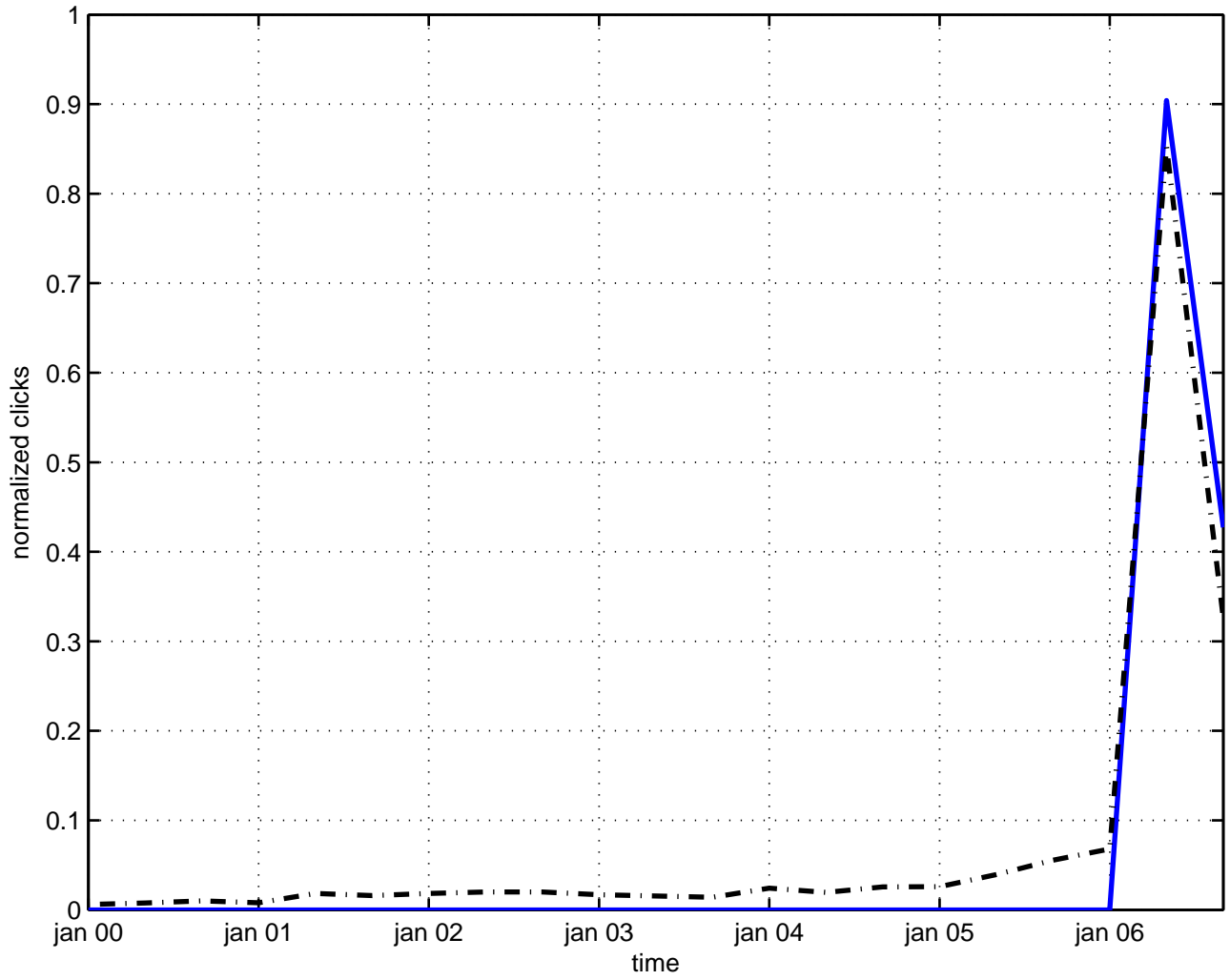
deconfinement temperature
