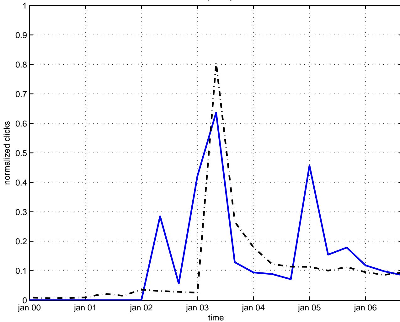
decay tachyon
