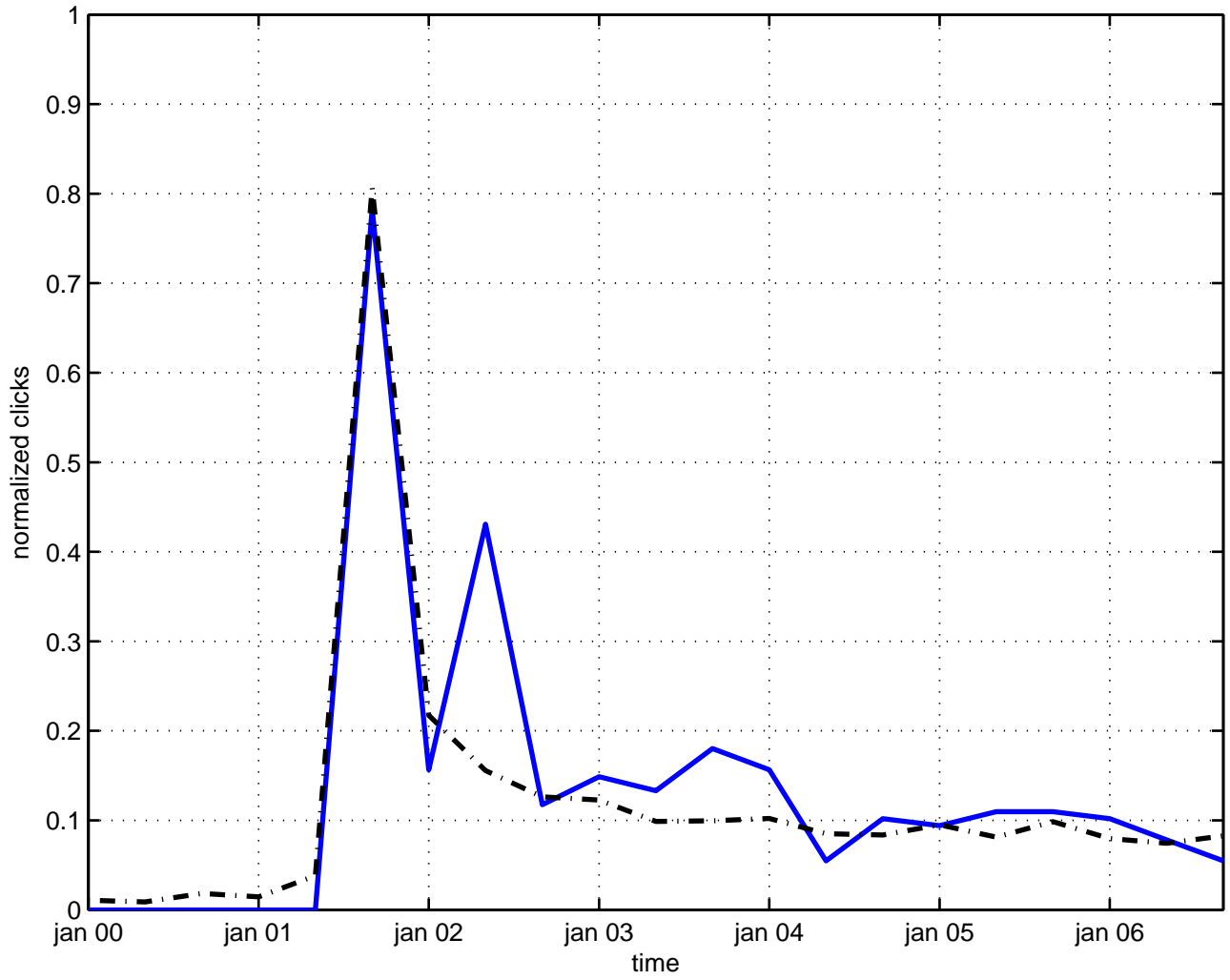
decay sphere
