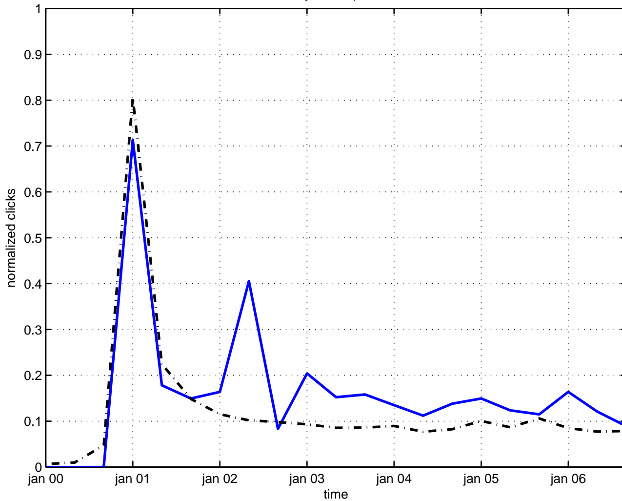
decay scalar particle
