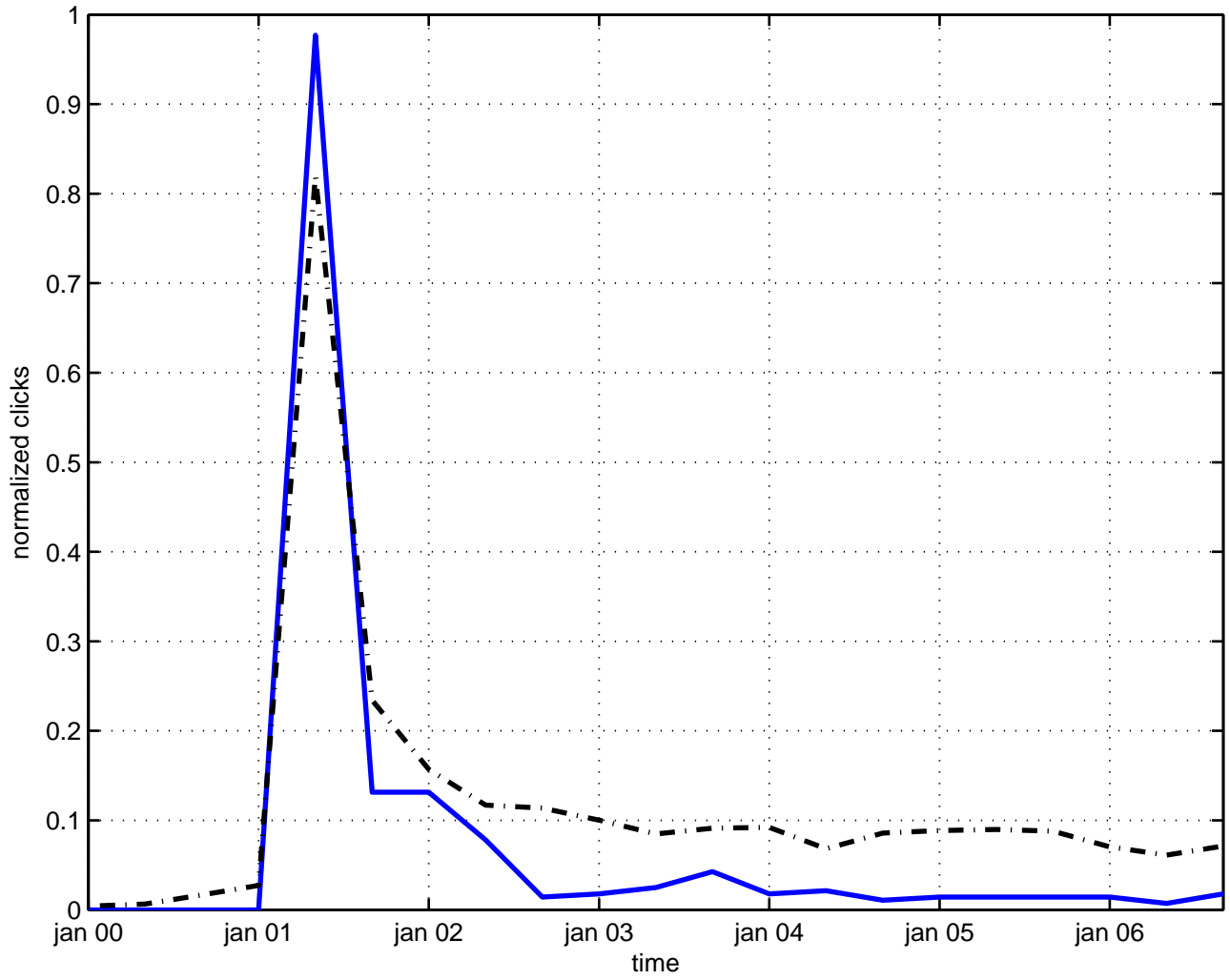
decay modes tachyon
