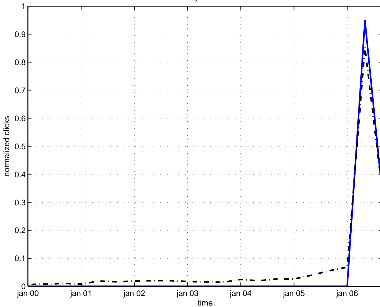
decay instanton
