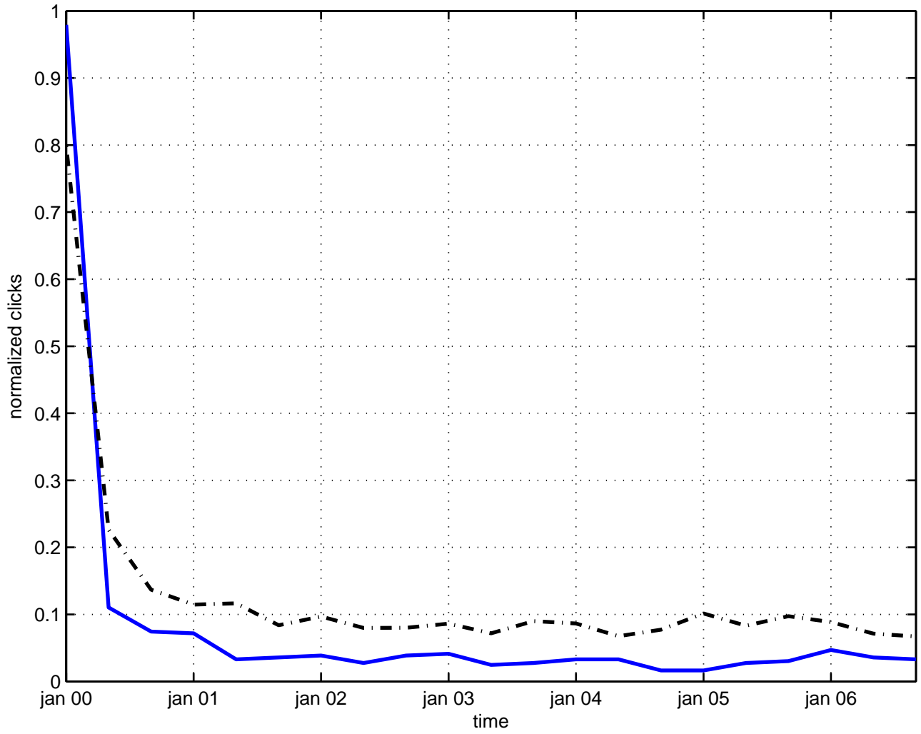
decay graviton
