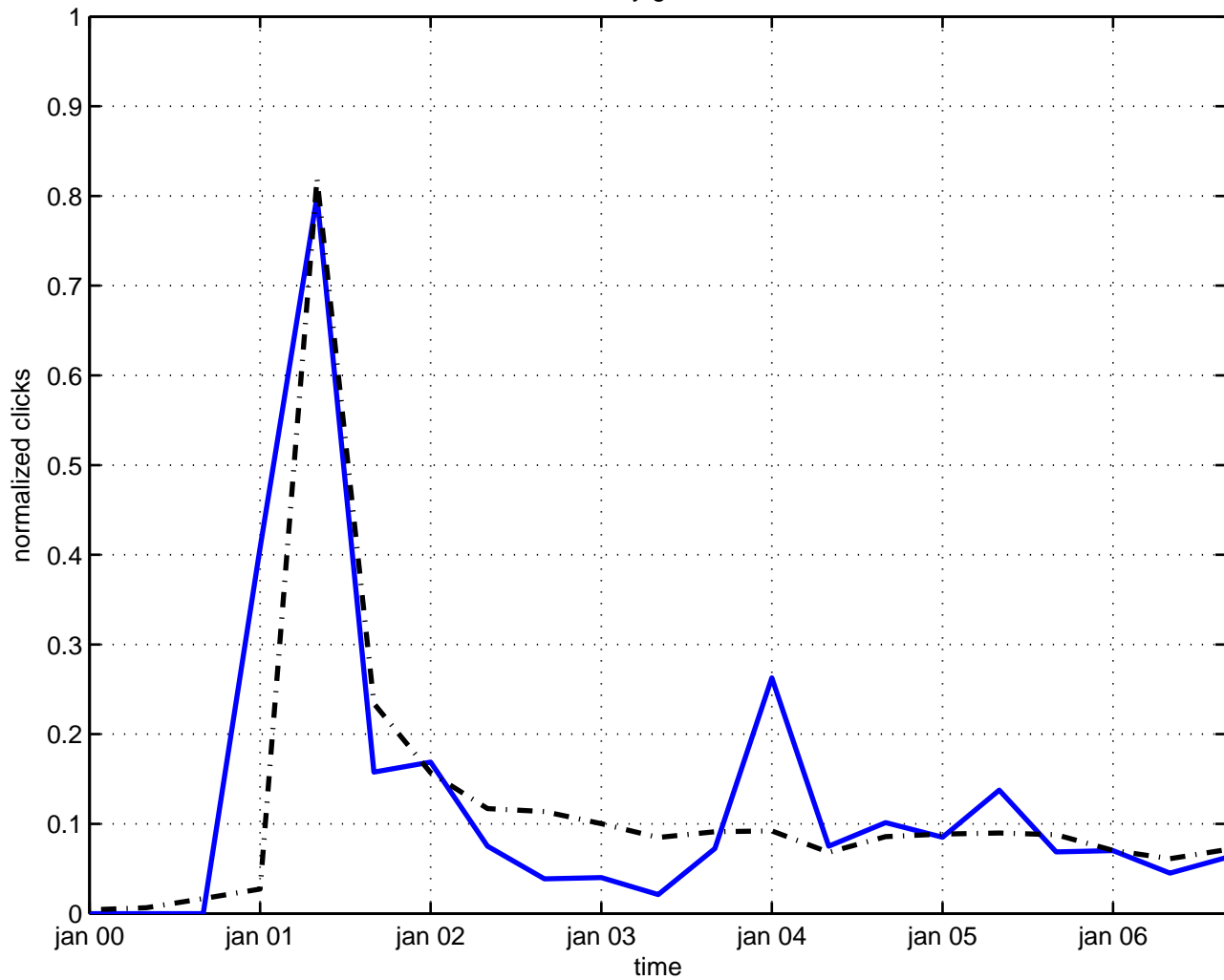
decay glueball
