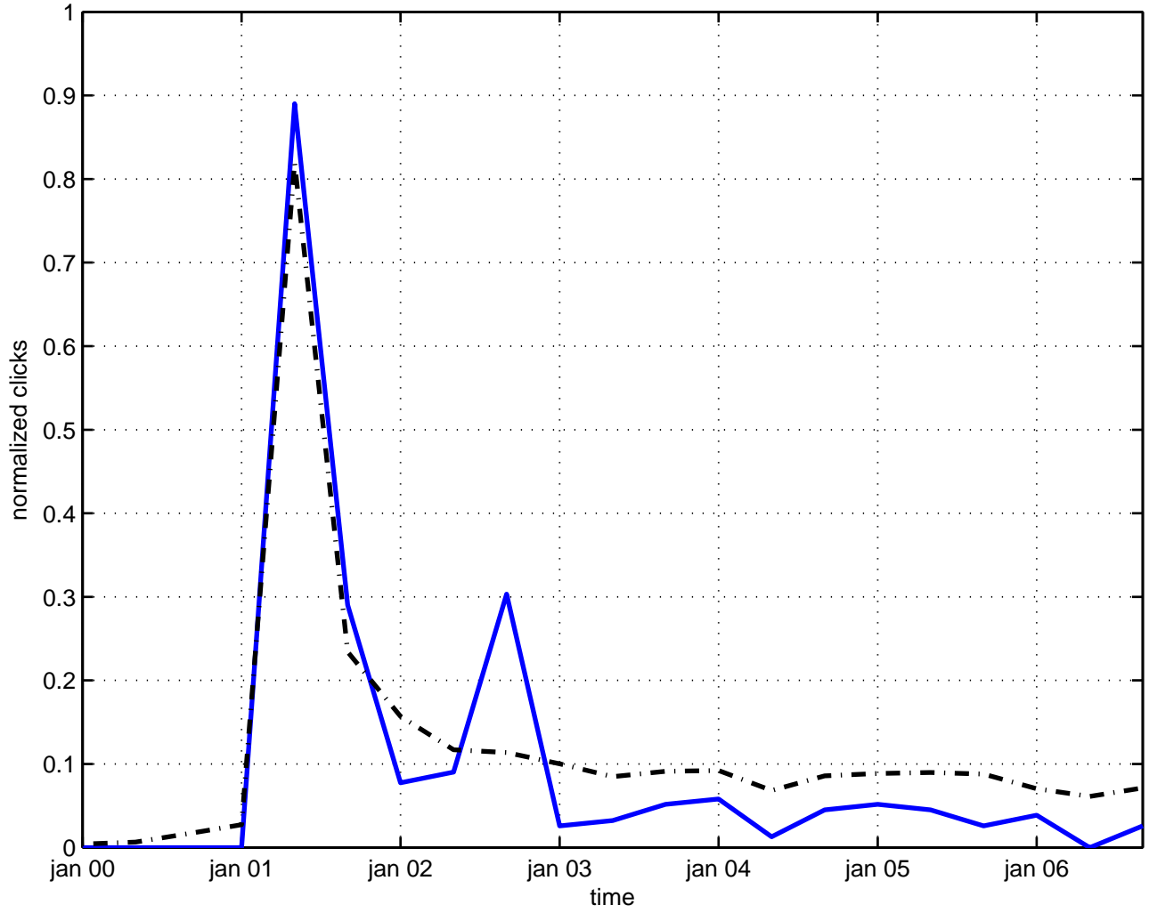
decay fundamental constant
