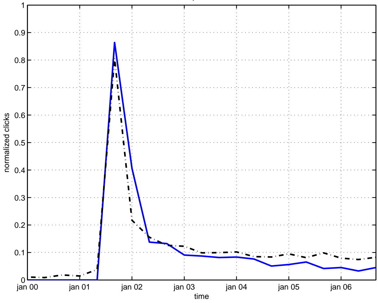
decay flux tube
