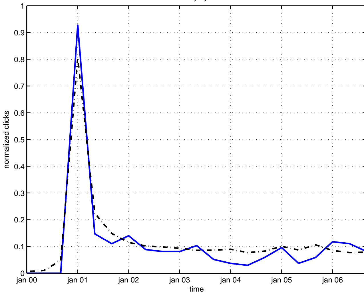
decay dyon
