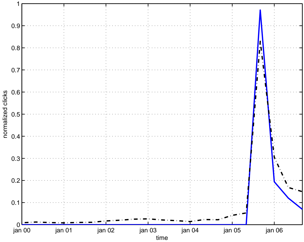
decay dilaton
