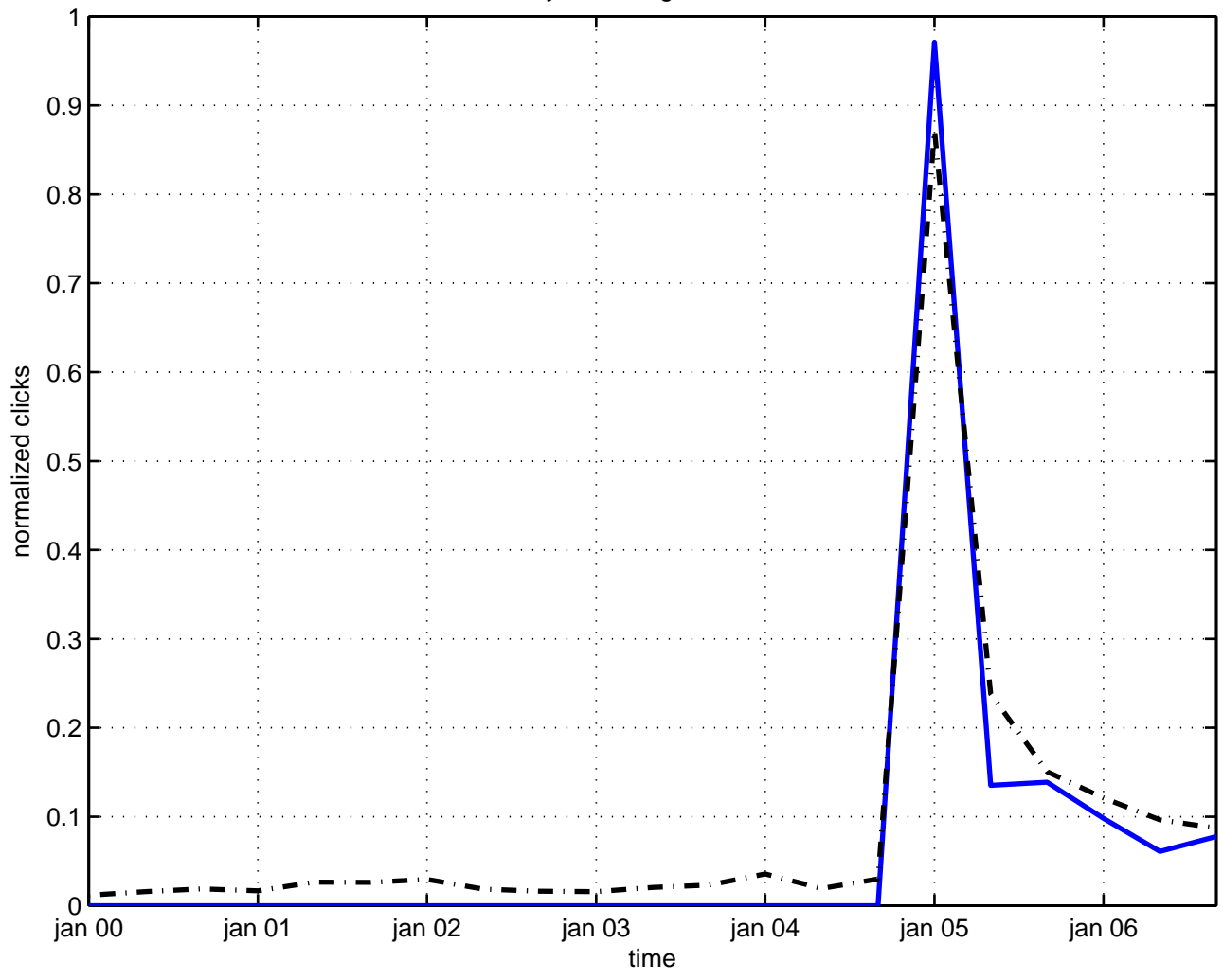
decay cosmological constant
