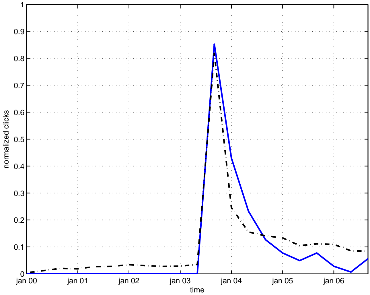
decay cosmic string
