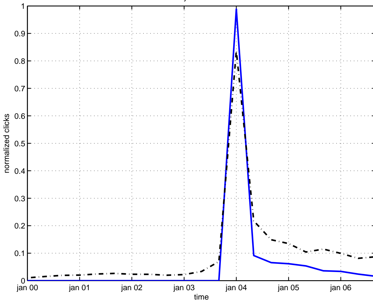
decay condensation
